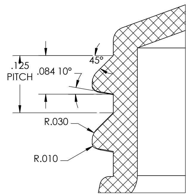
DETAIL E SCALE 8 : 1
