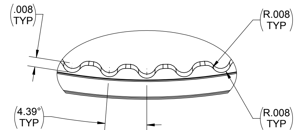
DETAIL B SCALE 20 : 1 (82 EQUALLY SPACED KNURLS)
