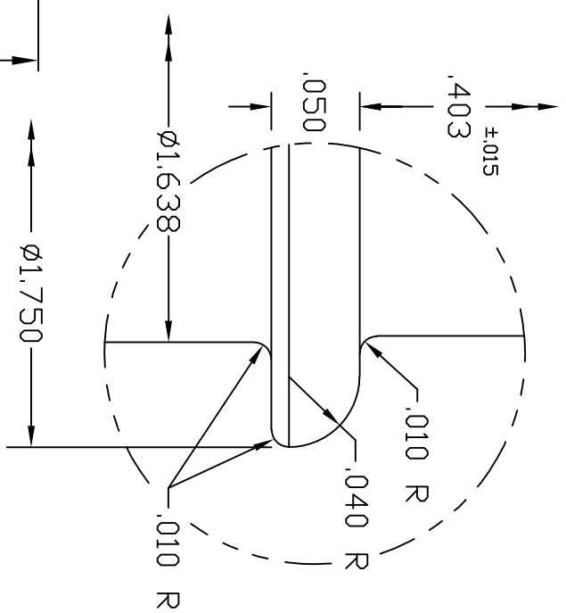
Bead Detail Scale 10 to 1
