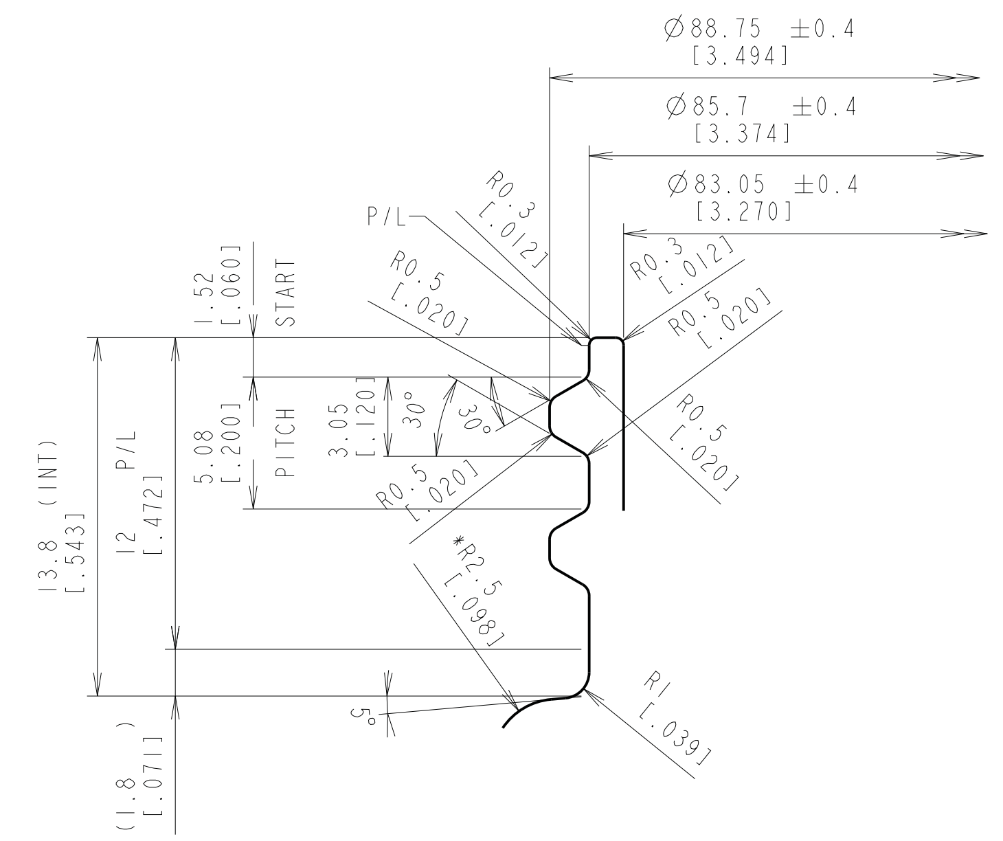
NECK DETAIL-SECTION A-A SCALE 5 TURN 1 1/8 PITCH 5.08 [0.200] CUTTER DIA 12.7 [0.500]
