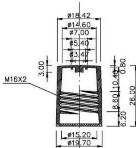
滚珠盖剖面 roll on cap cutaway diagram
