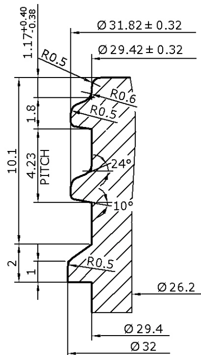
FINISH DETAIL S/5:1
