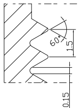
TUBE DETAIL SCALE 10:1
